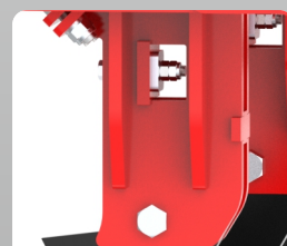
Shear Bolt Safety Mechanism
